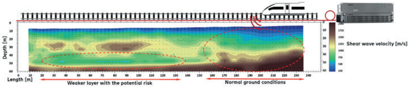
BBS solution in action: 2D shear velocity profile is presented under the rail track, with normal ground conditions on the right and zone of potential risk on the left
