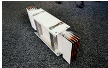
Figure 2: Schneider 2000A busway - sensor cable route planning and retrofitting by STS group
